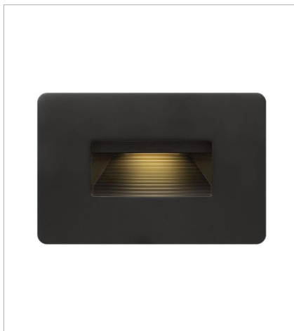
58508SK LED 2700K STEP LIGHT 120V ... 4.5" W, 3" H Integrated LED 4w LED *Included
