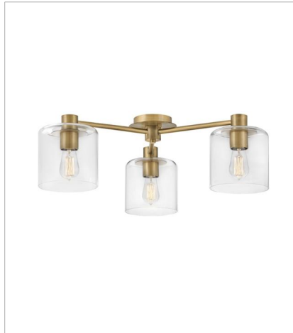
4514HB LARGE SEMI-FLUSH MOUNT 30" W, 9.8" H Socketed 3-10w Med. LED, 100w Equiv.
