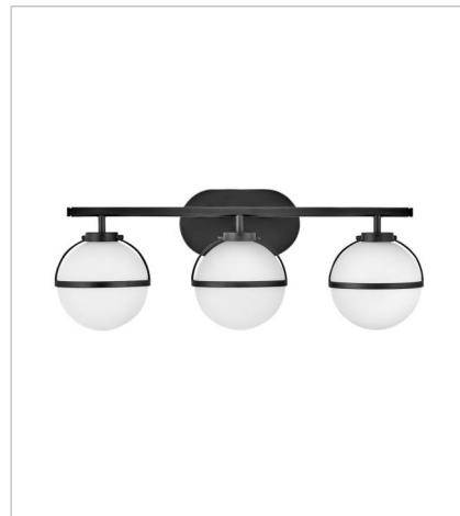
5663BK-LL THREE LIGHT VANITY 24" W, 9.3" H Socketed 3-5w G9 LED *Included
