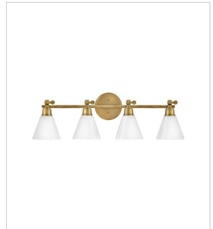
51184HB LARGE ADJUSTABLE FOUR LIGHT... 32" W, 10" H Socketed 4-10w Med. LED, 60w Equiv.
