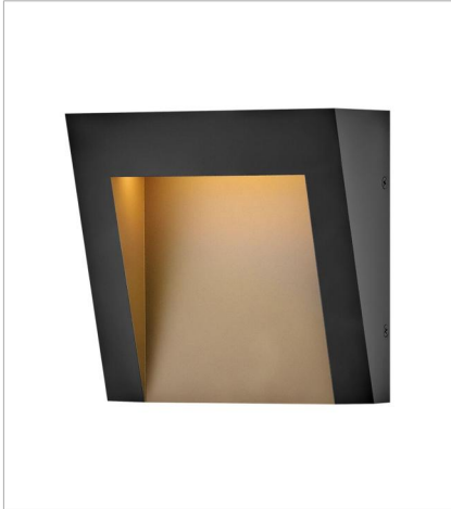
2140TK EXTRA SMALL WALL MOUNT LANTERN 7" W, 7" H Integrated LED 8.50w LED *Included
