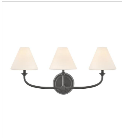
52493BLB-OP MEDIUM THREE LIGHT VANITY 24" W, 11.3" H Socketed 3-5w Cand. LED, 60w Equiv.
