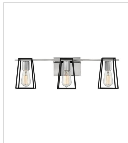
5163CM THREE LIGHTS VANITY 24" W, 7.5" H Socketed 3-14w Med. LED, 100w Equiv.
