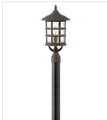
18610Z LARGE POST TOP OR PIER MOUN... 8" W, 20.5" H Socketed 1-12w Med. LED, 100w Equiv.
