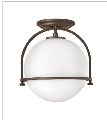
3403KZ SMALL SEMI-FLUSH MOUNT 11.5" W, 12.5" H Socketed 1-8w Med. LED, 100w Equiv.
