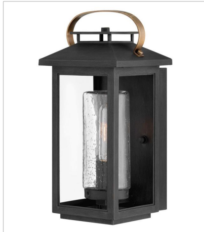
1160BK-LL SMALL WALL MOUNT LANTERN 6.5" W, 14" H Socketed 1-2w Med. LED *Included
