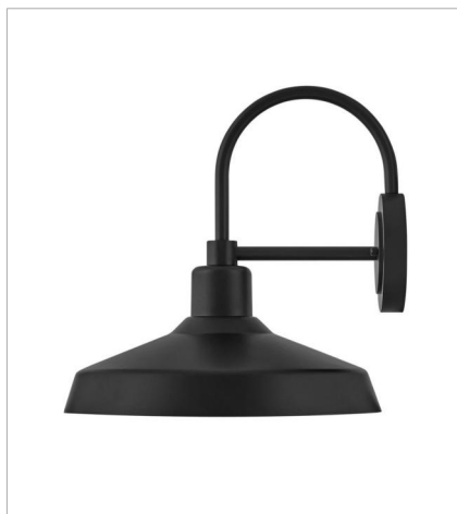
12070BK MEDIUM WALL MOUNT LANTERN 16" W, 16.5" H Socketed 1-14w Med. LED, 100w Equiv.
