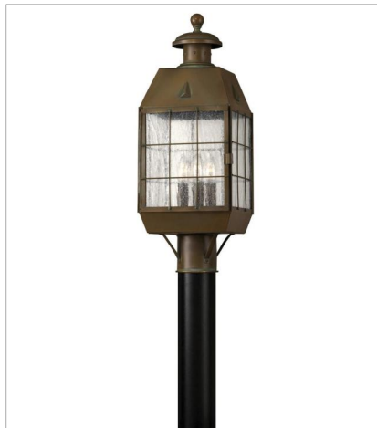
2371AS MEDIUM POST MOUNT LANTERN 7.5" W, 20.8" H Socketed 3-5w Cand. LED, 60w Equiv.
