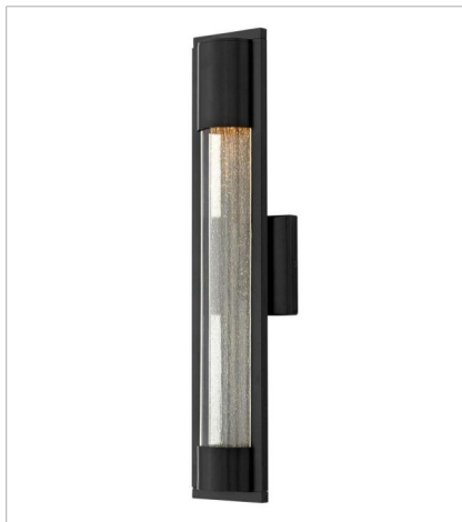
1224SK MEDIUM WALL MOUNT LANTERN 4.8" W, 22" H Socketed 1-7w GU10 LED, 50w Equiv.
